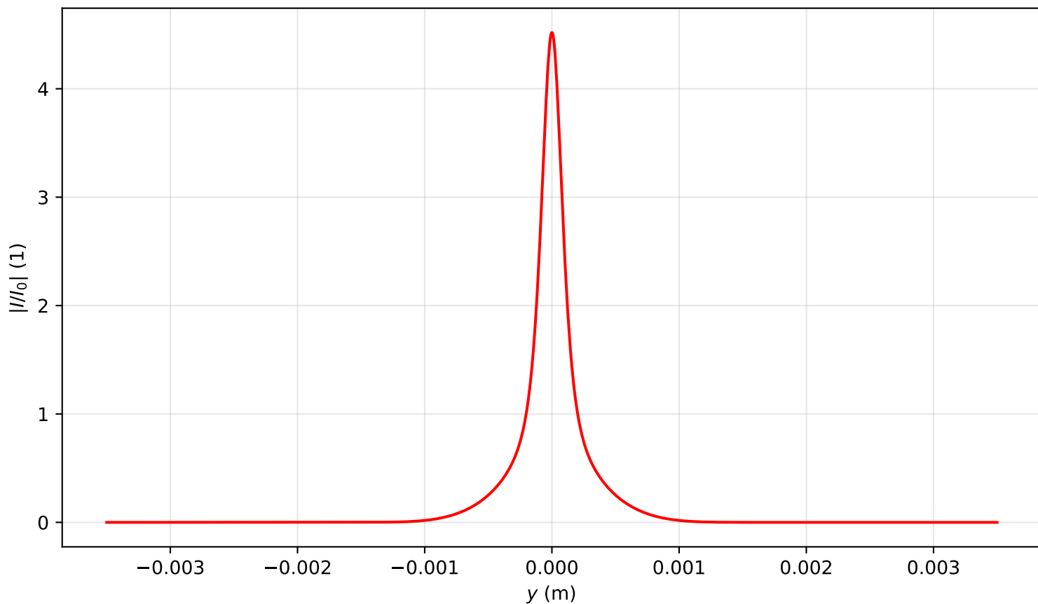
Intensity profile I(x=0, y, z=0.478)/I_0 , P_{in}=4.0P_{cr} , artificial time
